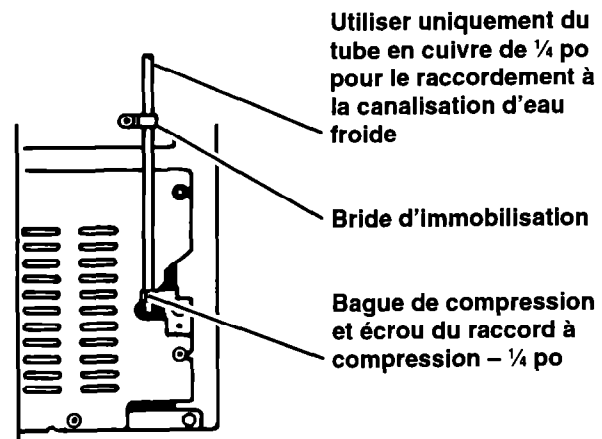
Style de valve #2
